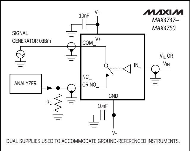
Figure 5. Off-Isolation/On-Channel Bandwidth
