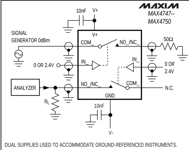
Figure 6. Crosstalk
