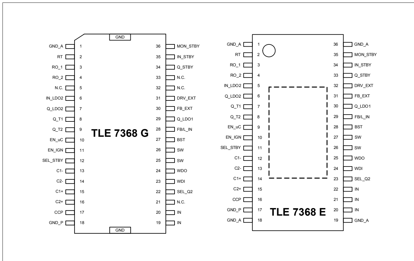
Figure 2 Pin Configuration
