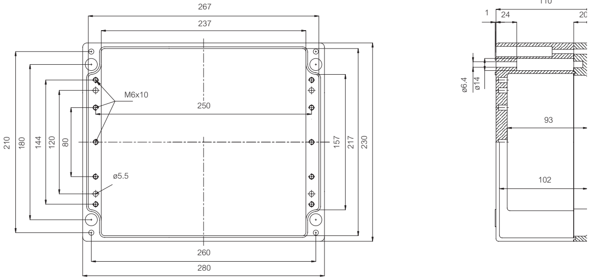
FIBOX ALUMINIUM AL 232811
