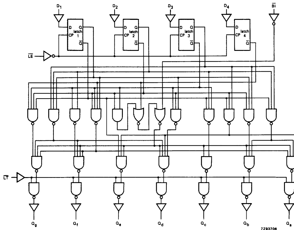
Fig.5 Logic diagram.
