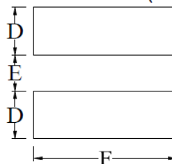
LAND PATTERNS(mm)
