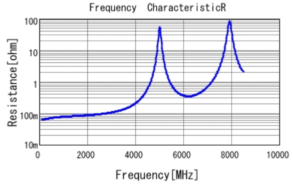
■ GQM1875C2E130JB12 R DCOV, 25degC
