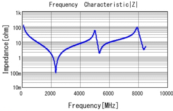
■ GQM1875C2E130JB12 |Z| DCOV, 25degC
