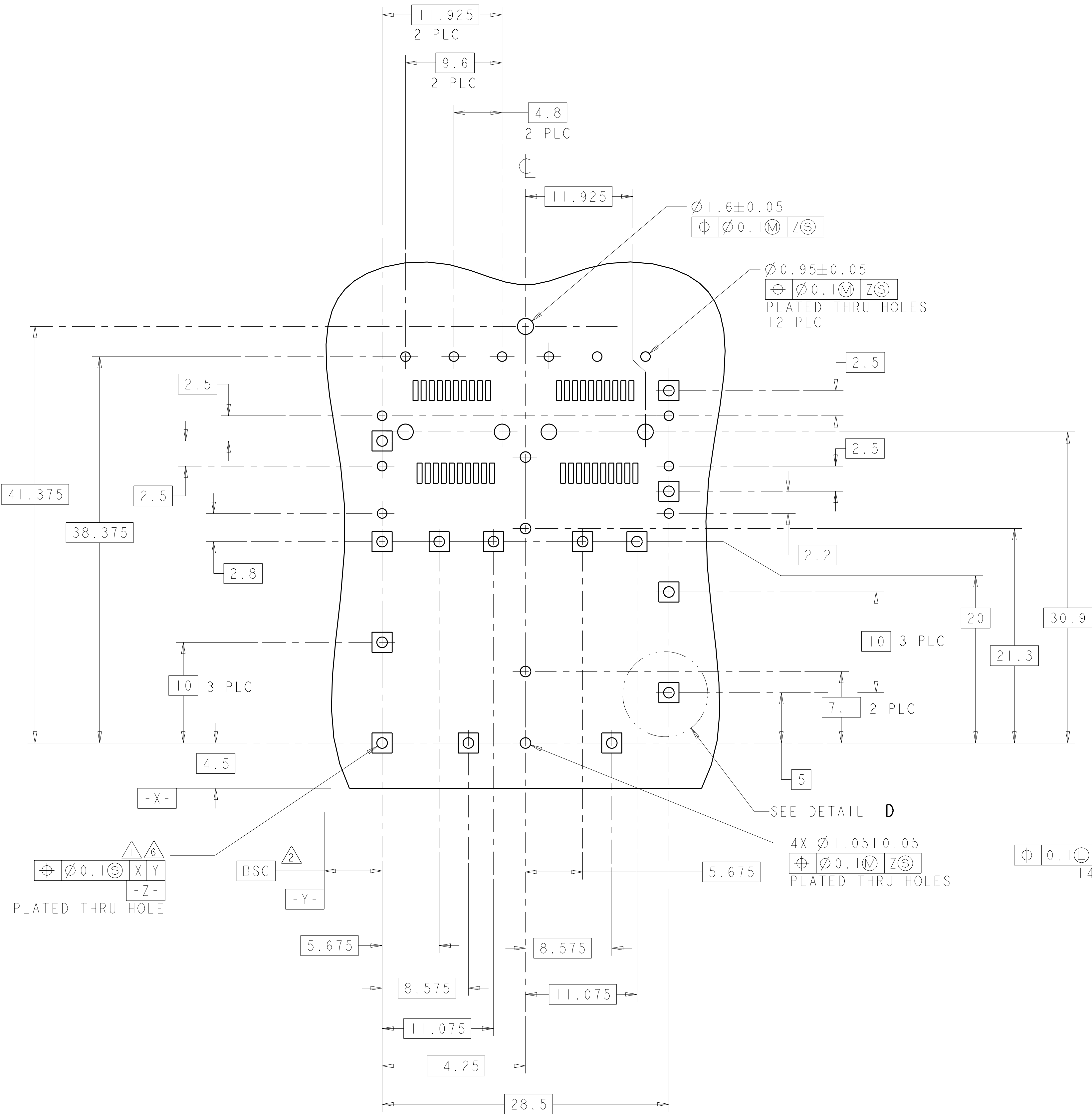
RECOMMENDED PC BOARD CONFIGURATION
