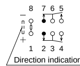
Single side stable (Deenergized condition)
