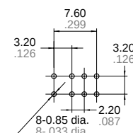
PC board pattern
