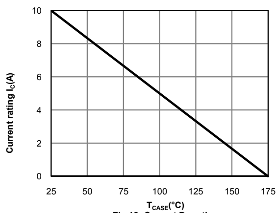
Fig 12: Current De-rating
