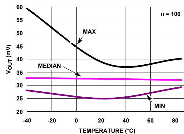
FIGURE 46. V_{OUT} LOW vs TEMPERATURE V_S = \pm 1.5V , R_L = 1k
