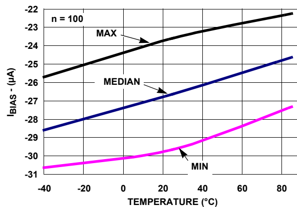
FIGURE 36. I_{BIAS-} vs TEMPERATURE V_S = \pm 2.5V
