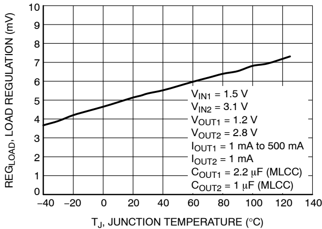
Figure 7. Load Regulation vs. Temperature – V OUT1 = 1.2 V
