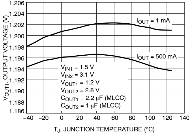
Figure 3. Output Voltage vs. Temperature – V OUT1 = 1.2 V
