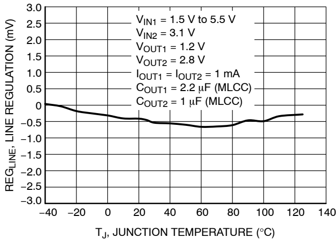
Figure 5. Line Regulation vs. Temperature – V OUT1 = 1.2 V
