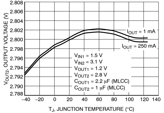
Figure 4. Output Voltage vs. Temperature – V OUT2 = 2.8 V
