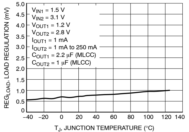
Figure 8. Load Regulation vs. Temperature – V OUT = 2.8 V
