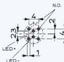
Drilling diagram
