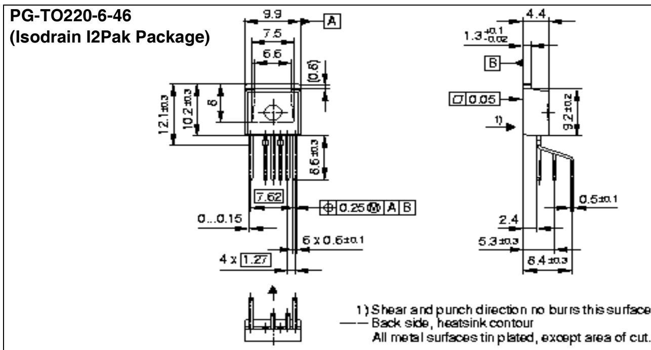
Figure 23 PG-TO220-6-46 (Pb-free lead plating Isodrain I2Pak Package)
