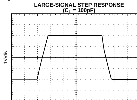
1μs/div Figure 20.
