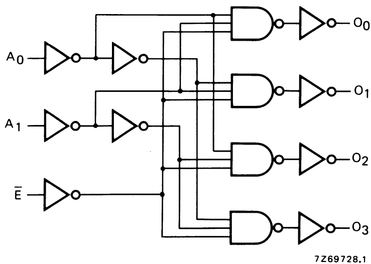
Fig.3 Logic diagram (one decoder/multiplexer).
