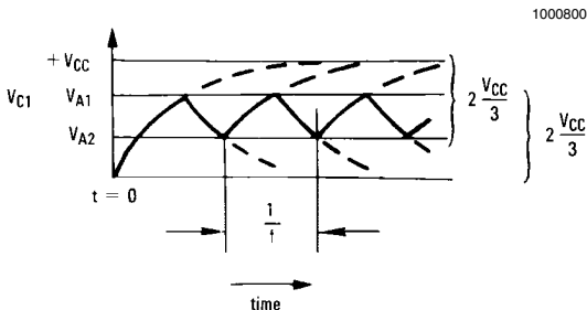
FIGURE 5. Squarewave Oscillator
