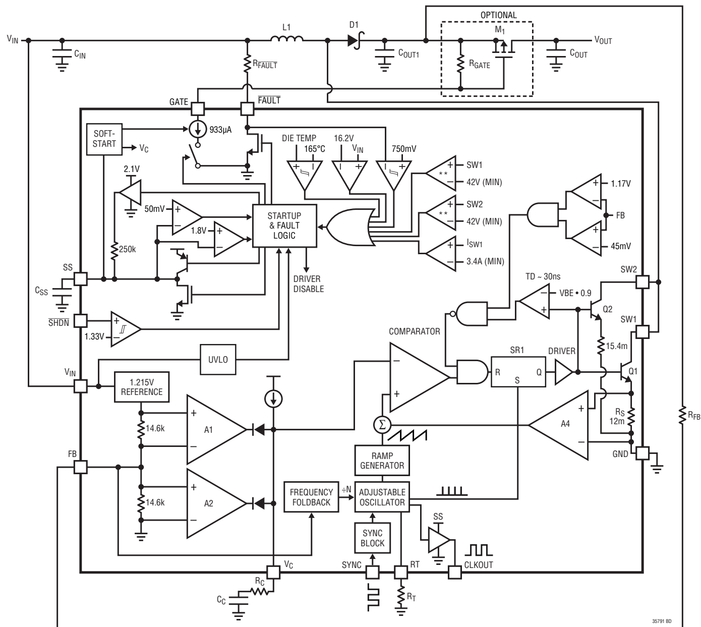
Figure 1. Block Diagram
