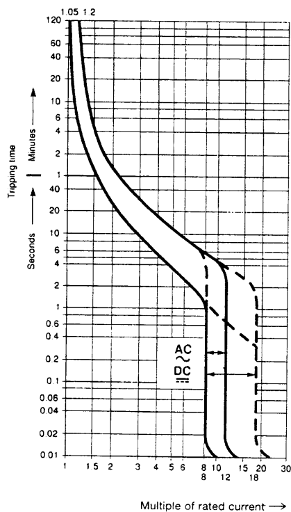
Tripping characteristic K I_n = 0.5 \dots 63 \text{ A} S 270
