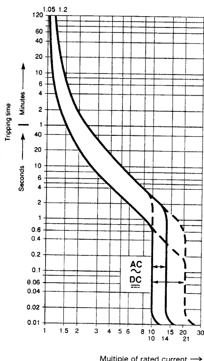
Tripping characteristic K I_n = 0.2 \dots 63 \text{ A} S 280
