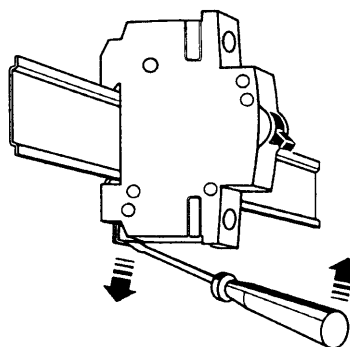
Fig. 2 Removal
