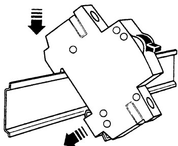
Fig. 1 Mounting
