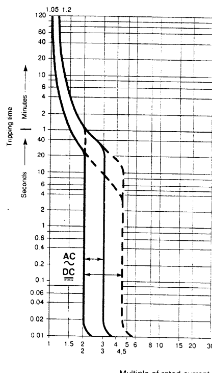
Tripping characteristic Z I_n = 0.5 \dots 63 \text{ A}
