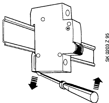
Fig. 2 Removal
