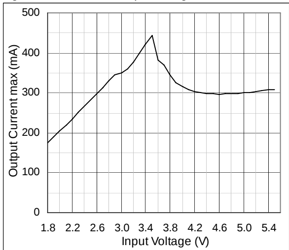
Figure 7. I_{OUT\ max} vs. Input Voltage
