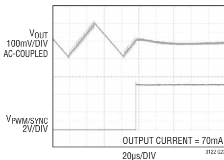
Burst Mode Operation to PWM Mode
