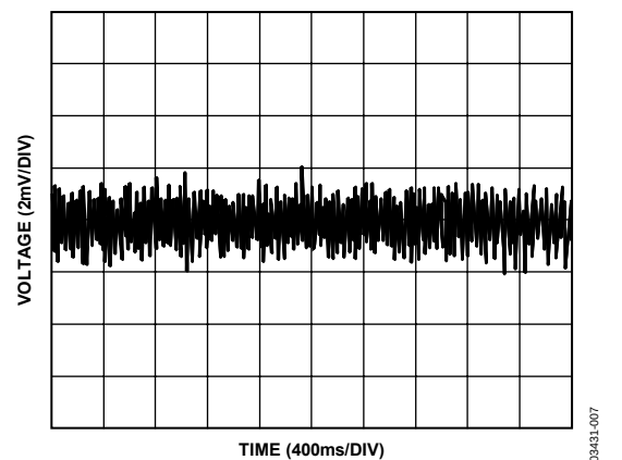
Figure 7. Typical Output Voltage Noise 0.1 Hz to 10 Hz
