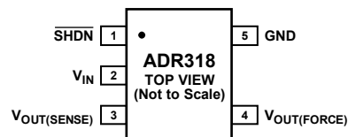
Figure 1. 5-Lead SOT-23
