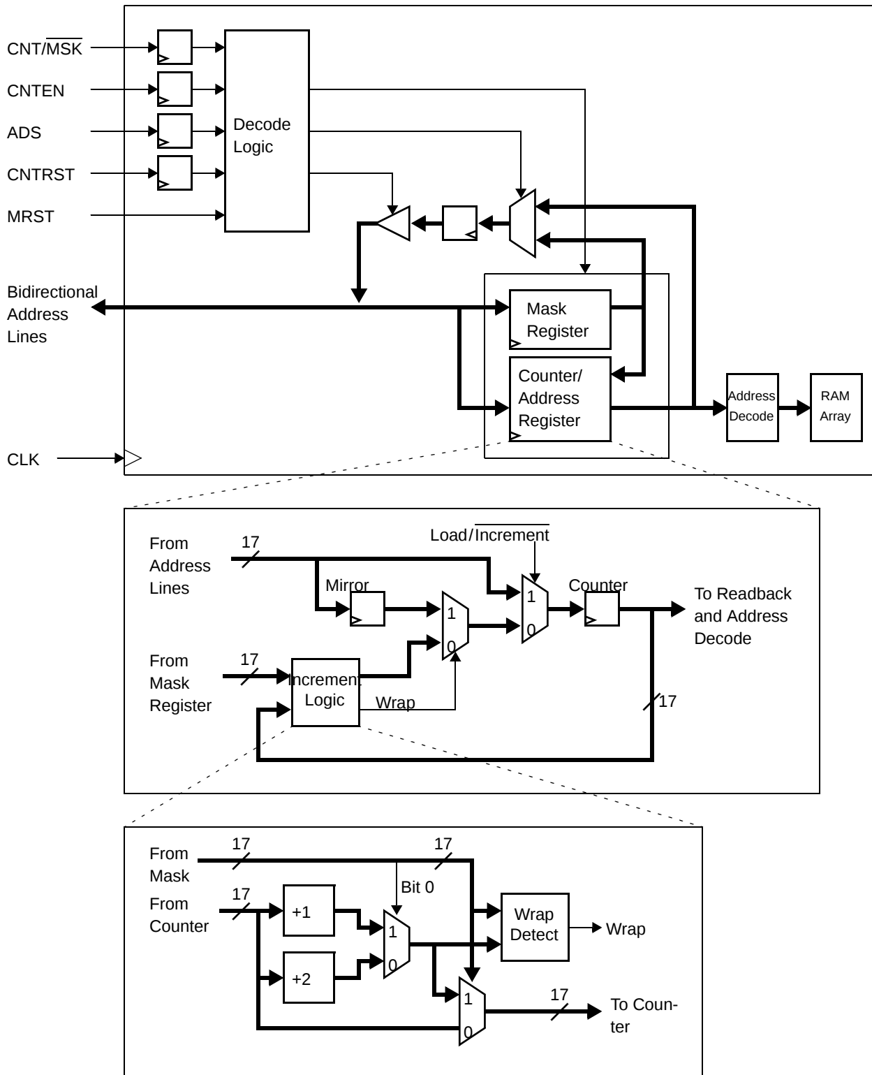
Figure 1. Counter, Mask, and Mirror Logic Block Diagram [30]
