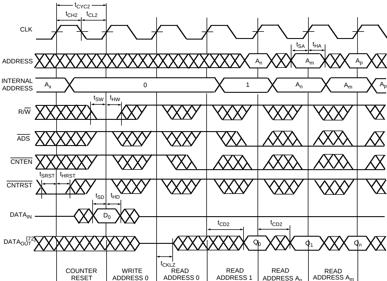
Figure 11. Counter Reset [59, 60]
