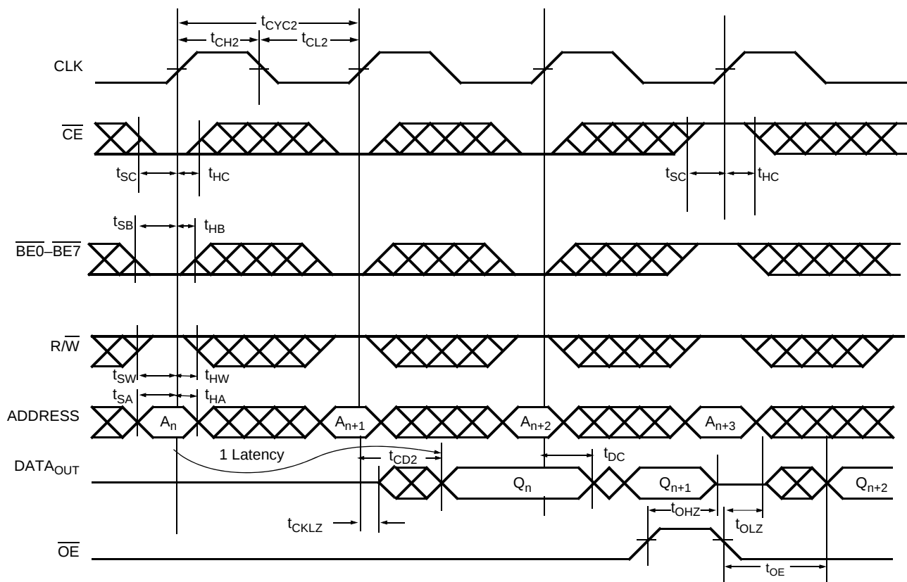
Figure 5. Read Cycle [43, 44, 45, 46, 47]
