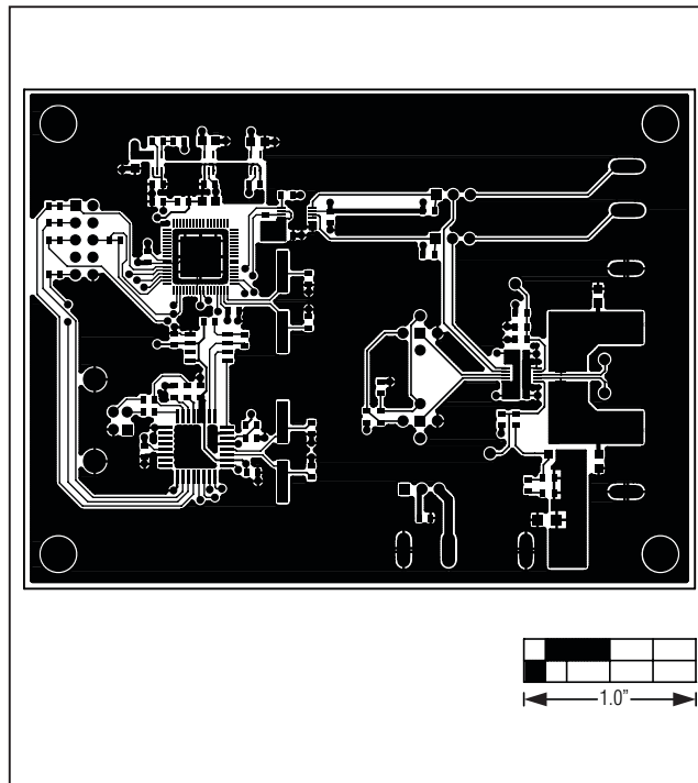
Figure 5. MAX9611 EV Kit PCB Layout—Component Side
