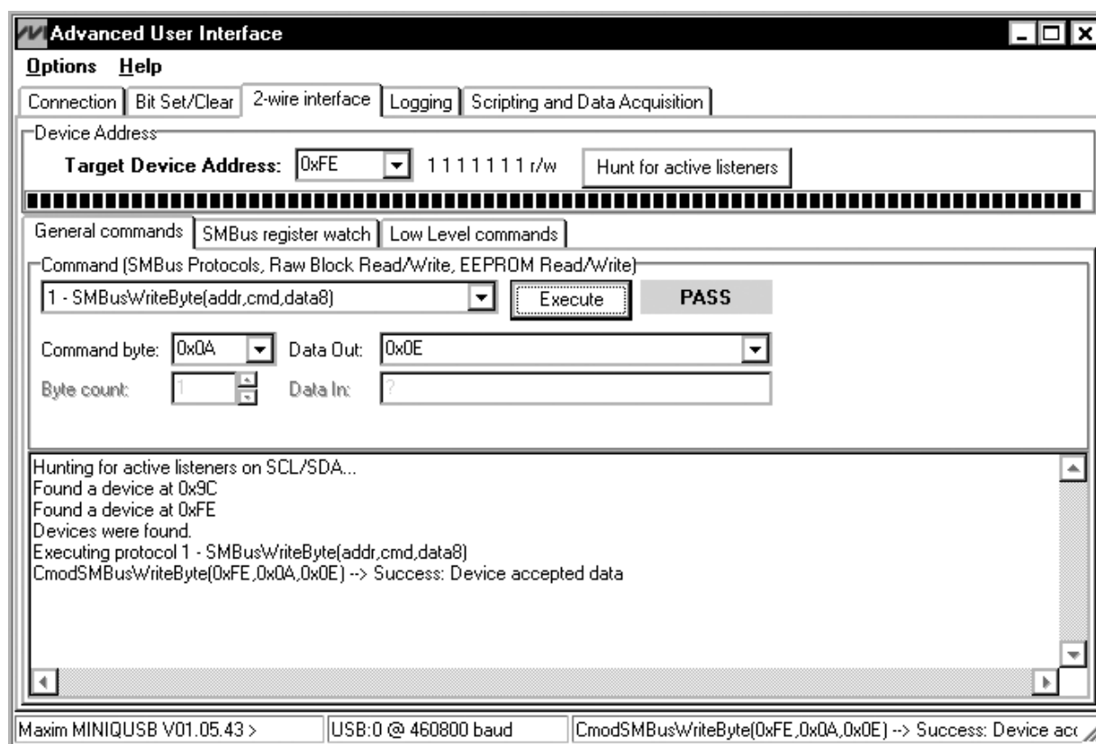
Figure 2. Example of an SMBusWriteByte Operation Using the Advanced User Interface
