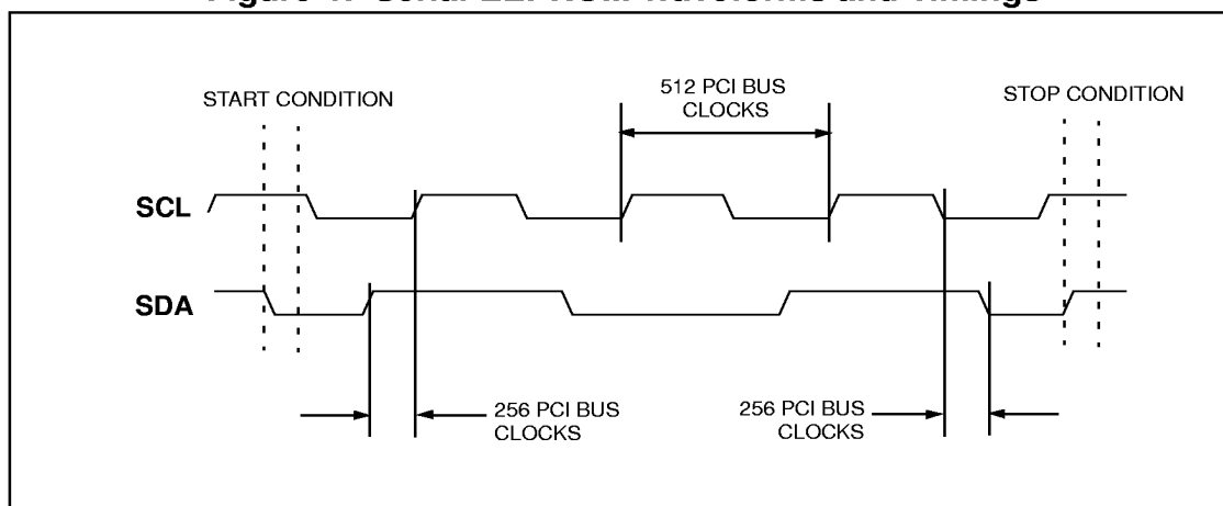
Figure 4: Serial EEPROM Waveforms and Timings
