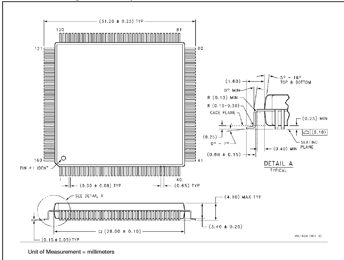
Figure 2: 160-pin EIAJ PQFP mechanical details
