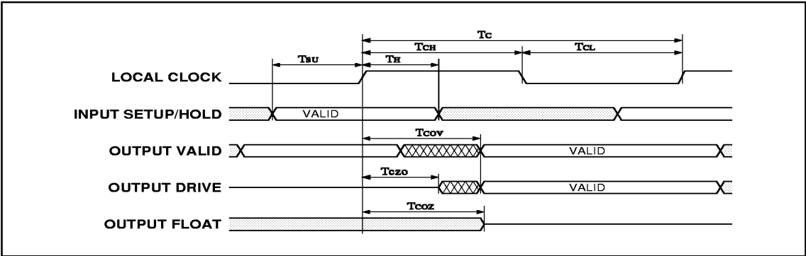
Figure 3: Clock and Synchronous Signals
