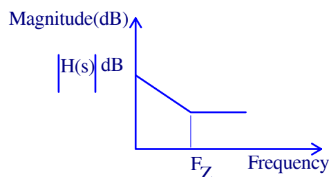
Fig. 15: Typical Type II Compensation and its Gain Plot
