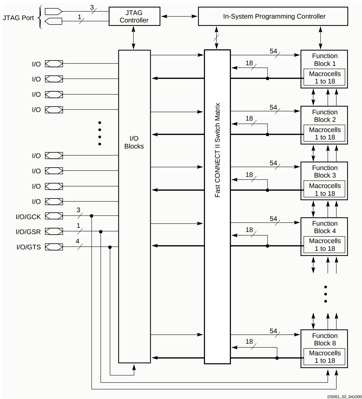
Figure 2: XC95144XV Architecture
