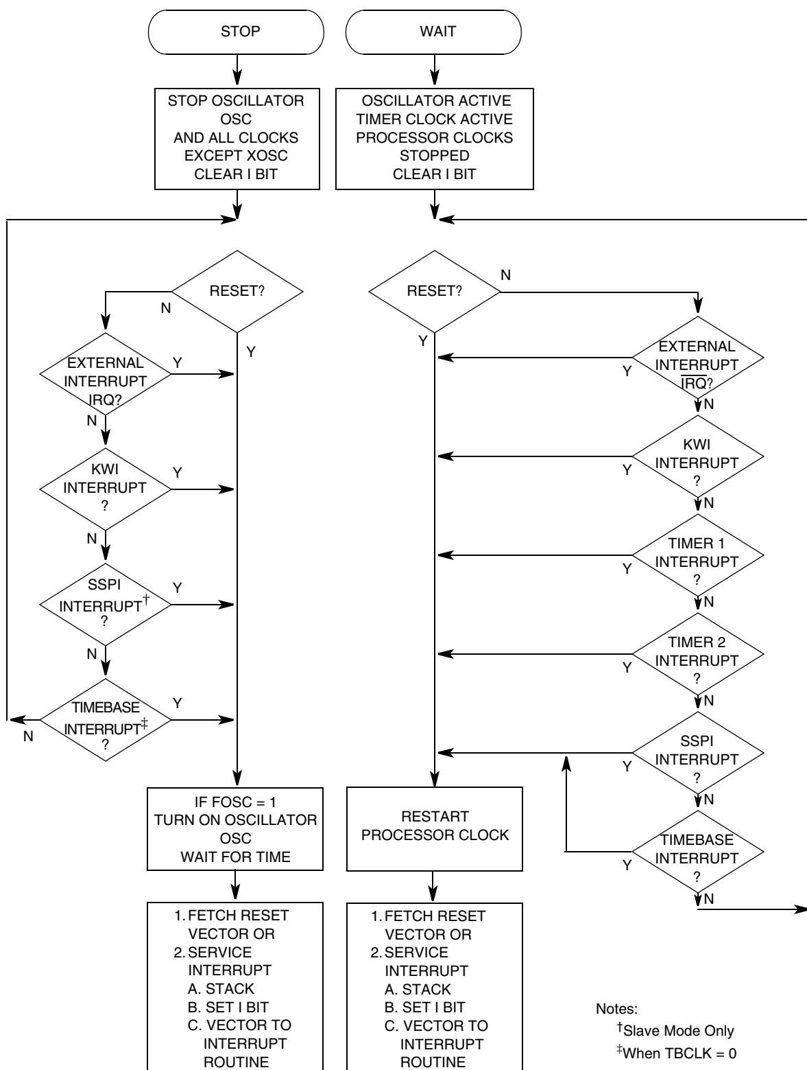
Figure 5-2. Stop/Wait Flowcharts
