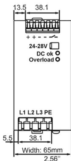
Fig. 24-1 Front view
