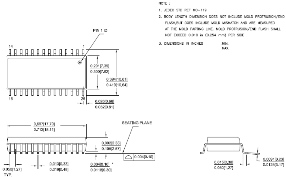
Figure 10. 28-pin SOIC Package Outline, 51-85026
