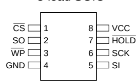
8-lead SOIC
