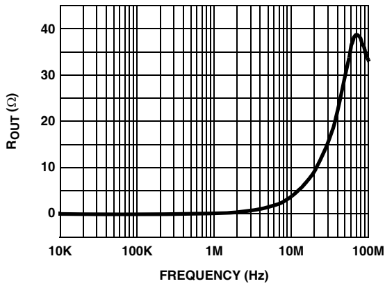
FIGURE 13. OUTPUT IMPEDANCE
