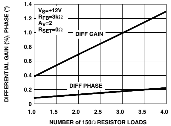
FIGURE 16. DIFFERENTIAL GAIN/PHASE, F_O = 3.58MHz (2/3 POWER MODE)
