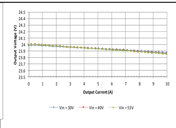
V_o = 24V Typical load regulation
