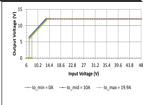
Vo=12V Typical Output Voltage vs. Input Voltage Characteristics
