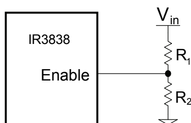
Fig. 15. Using Enable pin for UVLO implementation
