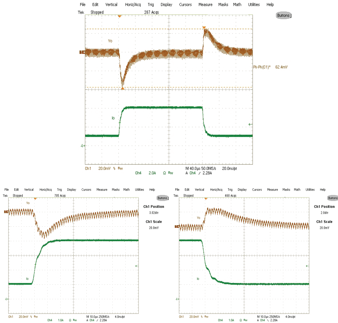
Fig. 28: Transient Response 1A-4A load (0.5A/us) Ch_1:V_{out} , Ch_4:I_o
