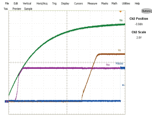
Fig. 23: Start up at 10A Load (Note 6) Ch 1 :V out Ch 2 :PGood Ch 3 :Vcc Ch 4 : V in
