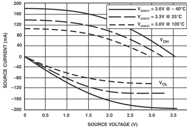
Figure 40. Driver Type A Current ( 3.3V_{DDEXT}/V_{DDMEV} )
