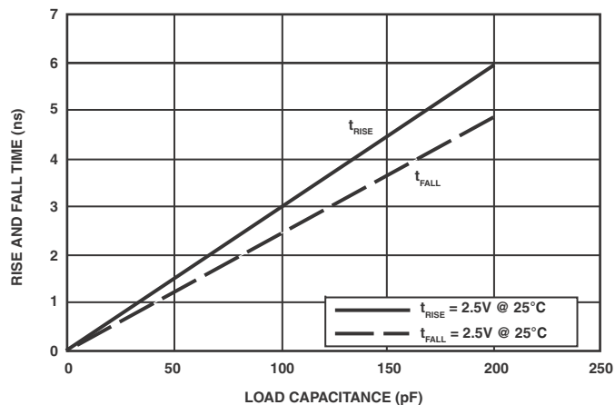
Figure 62. Driver Type B Typical Rise and Fall Times (10%–90%) vs. Load Capacitance ( 2.5V V_{DDEXT}/V_{DDMEM} )
