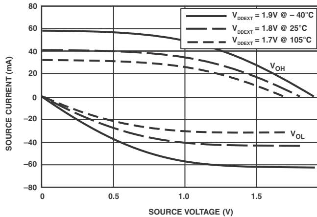
Figure 42. Driver Type A Current ( 1.8V_{DDEXT}/V_{DDMEV} )
