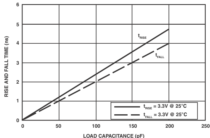
Figure 63. Driver Type B Typical Rise and Fall Times (10%–90%) vs. Load Capacitance ( 3.3V V_{DDEXT}/V_{DDMEM} )
