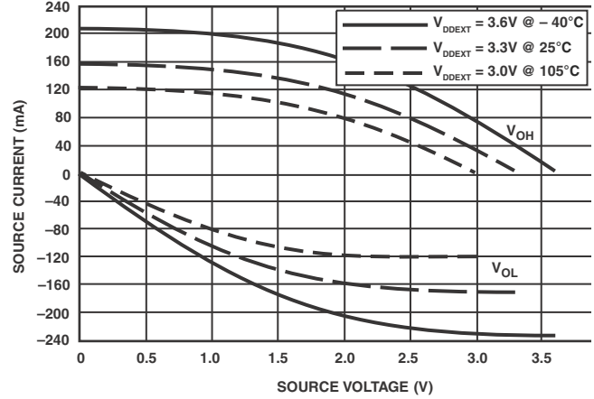
Figure 43. Driver Type B Current ( 3.3V_{DDEXT}/V_{DDMEV} )
