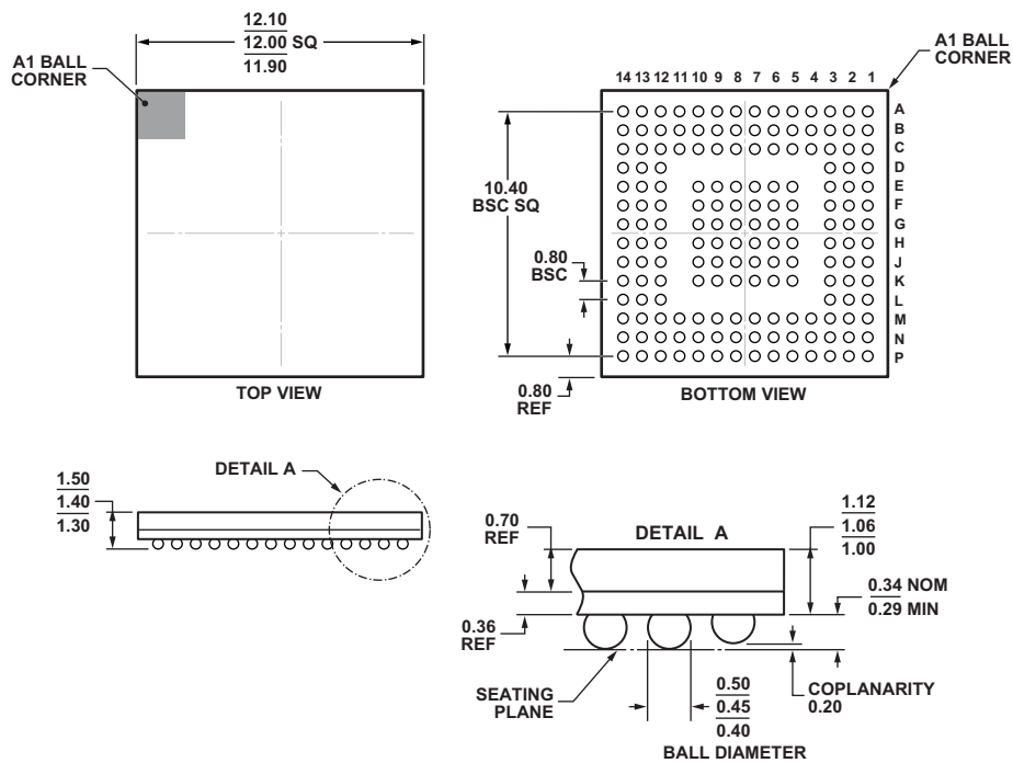
COMPLIANT TO JEDEC STANDARDS MO-275-GGAB-1. Figure 75. 168-Ball Chip Scale Package Ball Grid Array [CSP_BGA] (BC-168-1) Dimensions shown in millimeters
