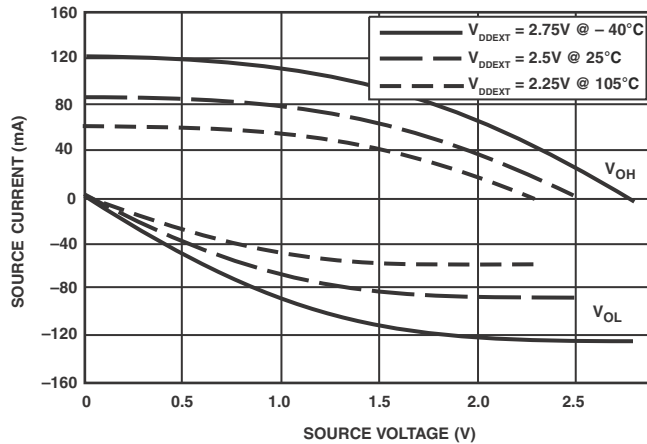
Figure 41. Driver Type A Current ( 2.5V_{DDEXT}/V_{DDMEV} )
