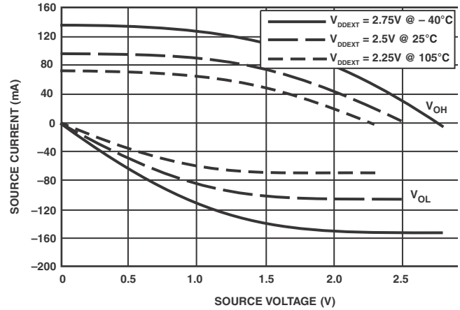
Figure 44. Driver Type B Current ( 2.5V_{DDEXT}/V_{DDMEV} )
