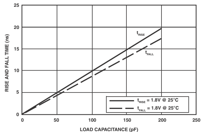
Figure 64. Driver Type C Typical Rise and Fall Times (10%–90%) vs. Load Capacitance ( 1.8V V_{DDEXT}/V_{DDMEM} )
