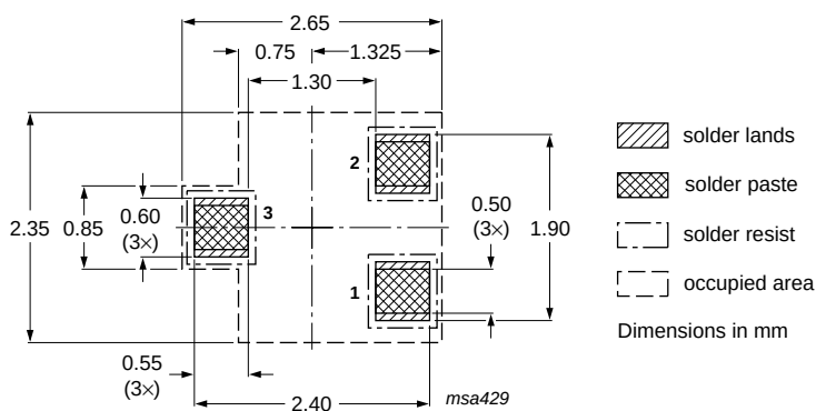
Fig 18. Reflow soldering footprint BAV70W (SOT323/SC-70)
