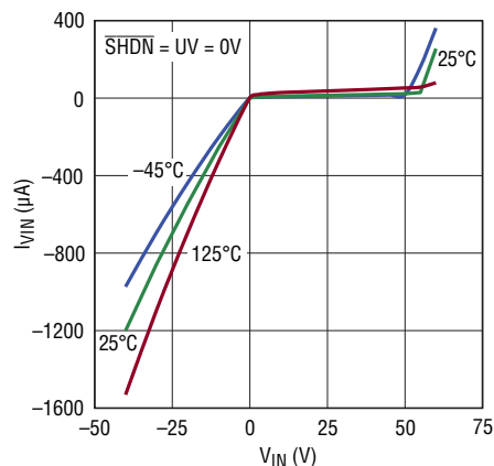
V_{IN} Current vs V_{IN} (-40 to 60V)
