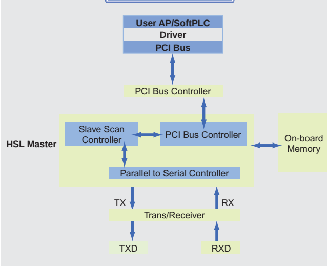
Block Diagram
