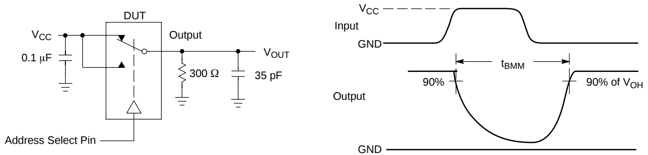
Figure 19. t_{\text{BBM}} (Time Break-Before-Make)
