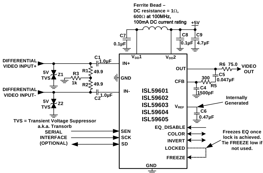
FIGURE 45. APPLICATION CIRCUIT FOR UTP CABLE
