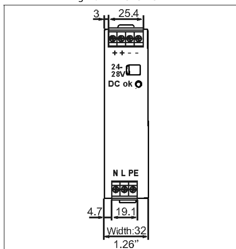
Fig. 20-1 Front view
