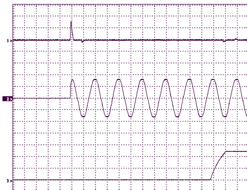
Fig. 5-1 Typical input inrush current behavior
