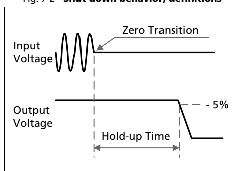
Fig. 7-2 Shut-down behavior, definitions
