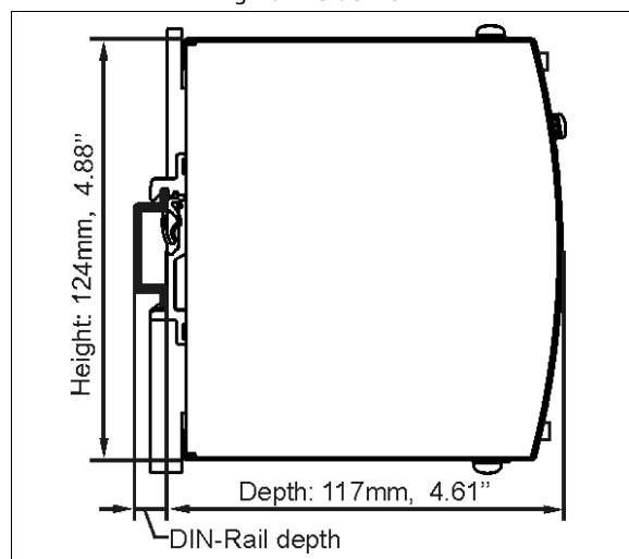
Fig. 20-2 Side view
