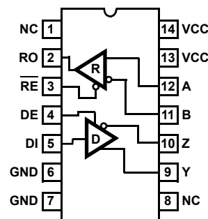
ISL32490E, ISL32493E, ISL32496E (14 LD SOIC) TOP VIEW
