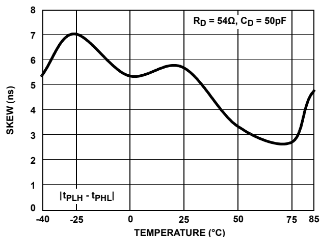
FIGURE 18. DRIVER DIFFERENTIAL SKEW vs TEMPERATURE (ISL32490E, ISL32492E)
