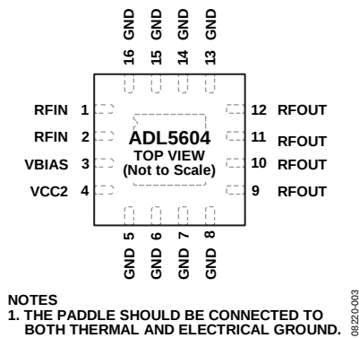
Figure 3. Pin Configuration
