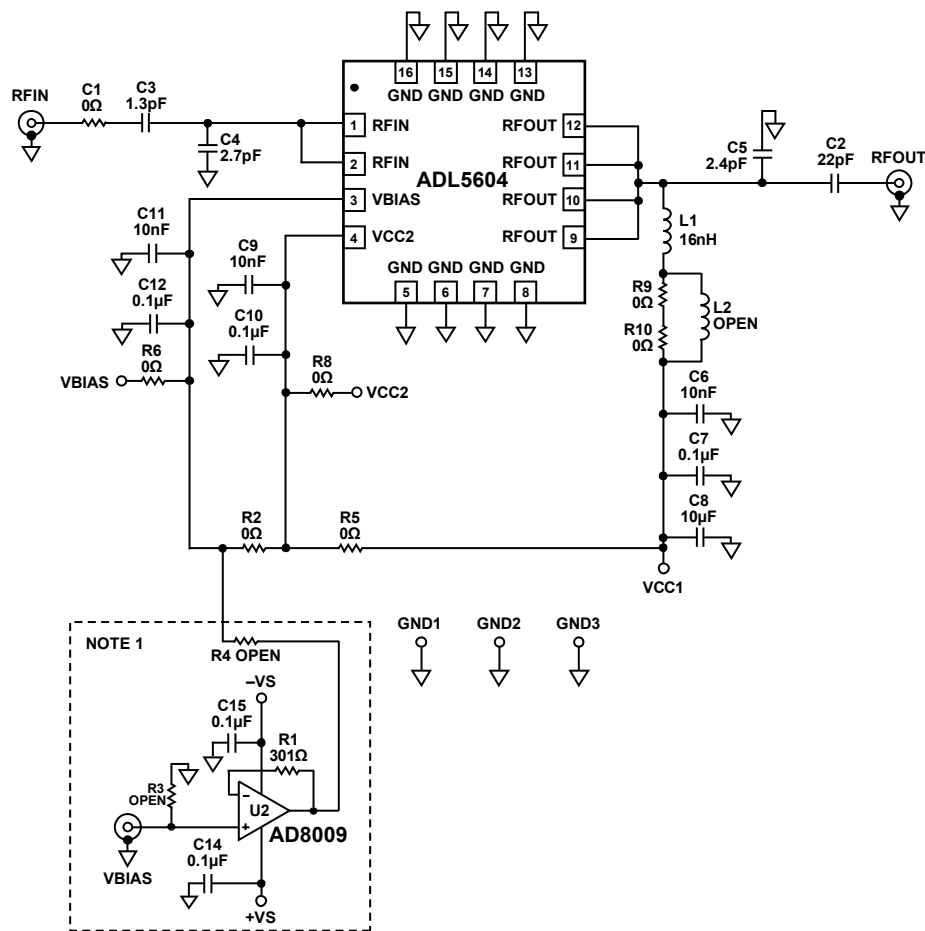
Figure 36. Basic Connections
