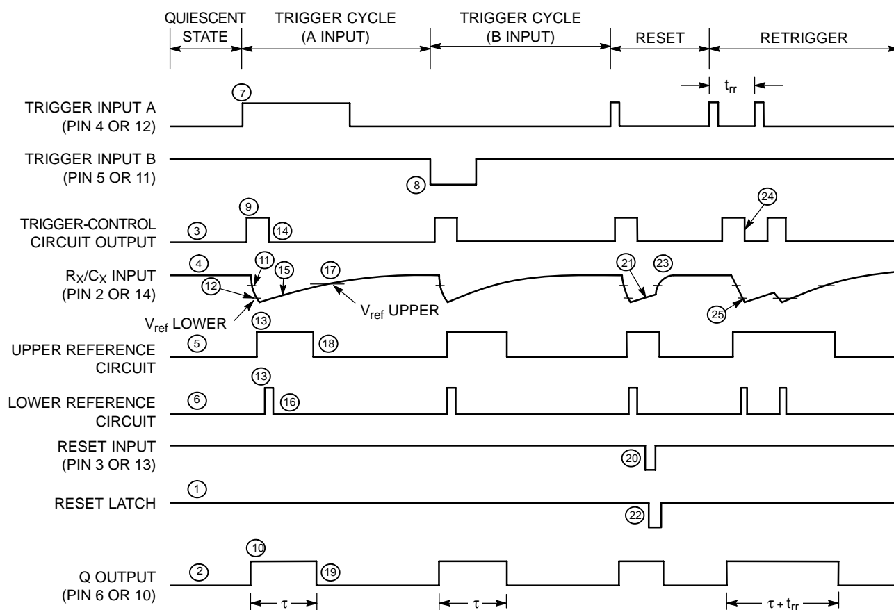
Figure 12. Timing Diagram
