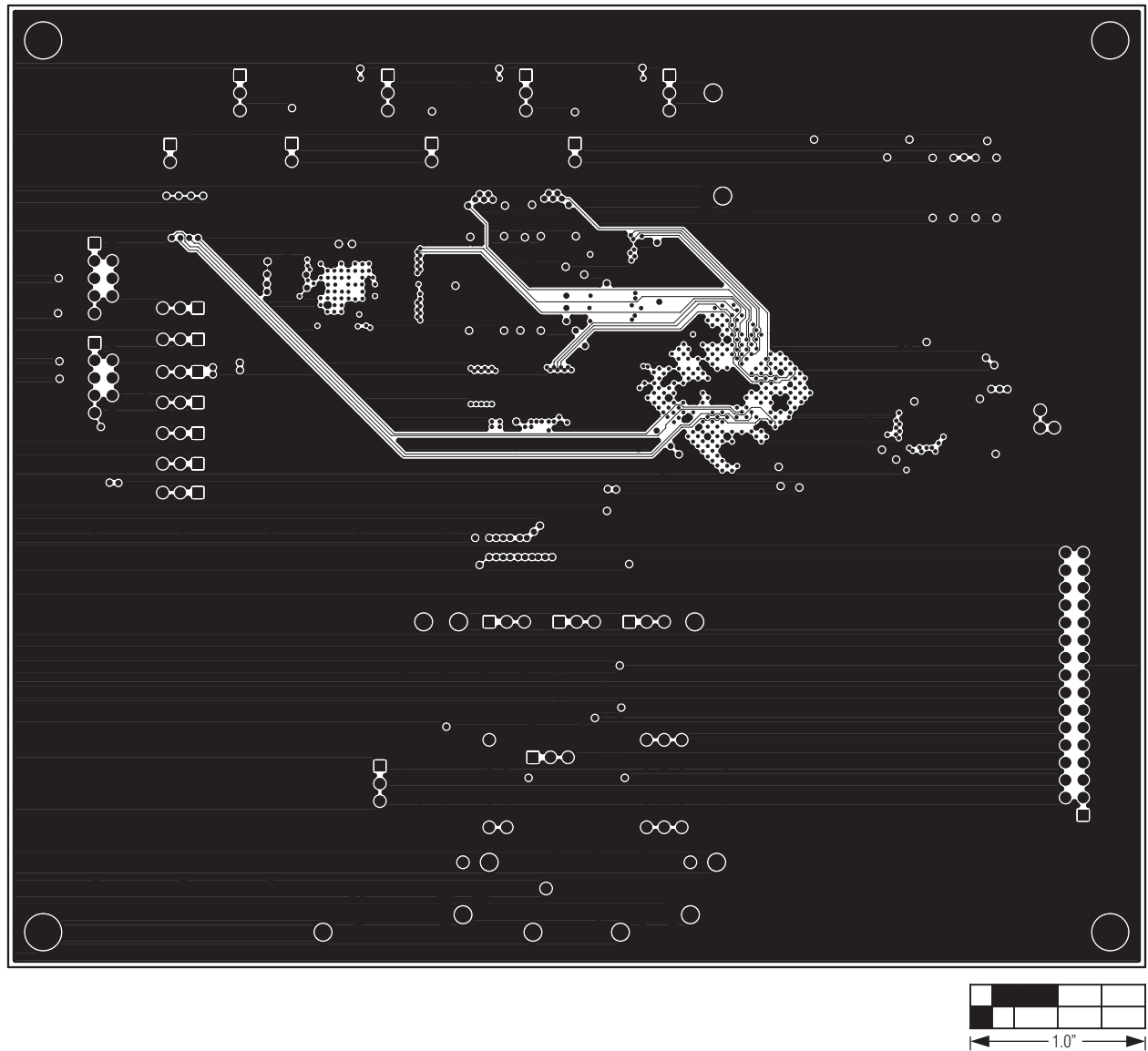
Figure 16. MAX11105 EV Kit PCB Layout—Layer 9
