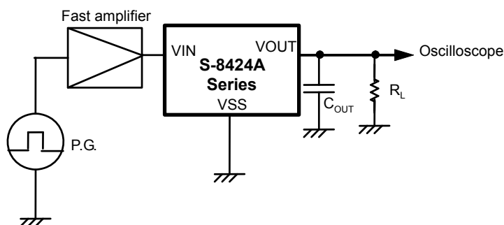
Figure 11 Test Circuit
