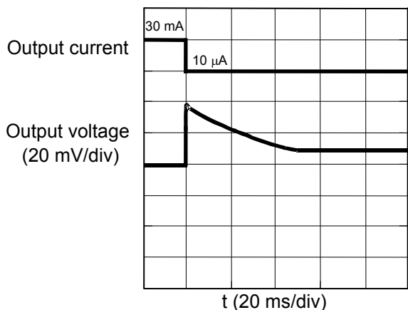
Figure 21 Ringing Waveform due to Load Variation (VRO Pin)
