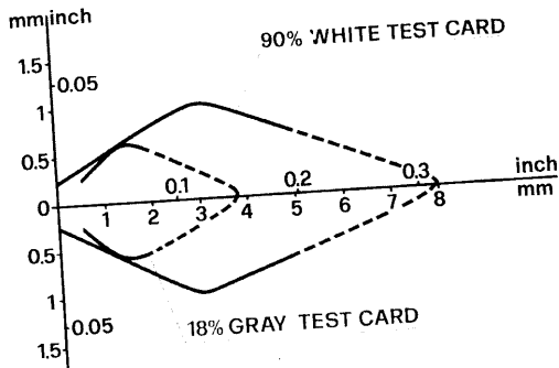
OF-26/OF-28 Proximity scanner
