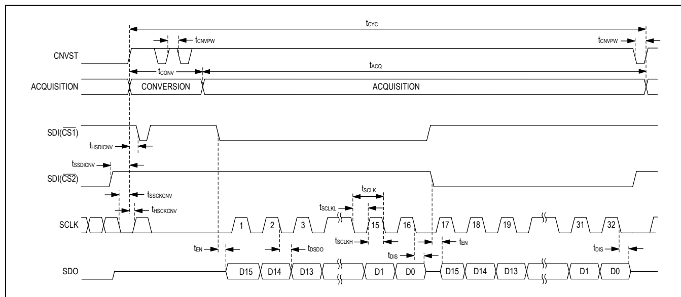
Figure 10. \overline{\text{CS}} Mode 4-Wire, No-Busy Indicator Serial Interface Timing
