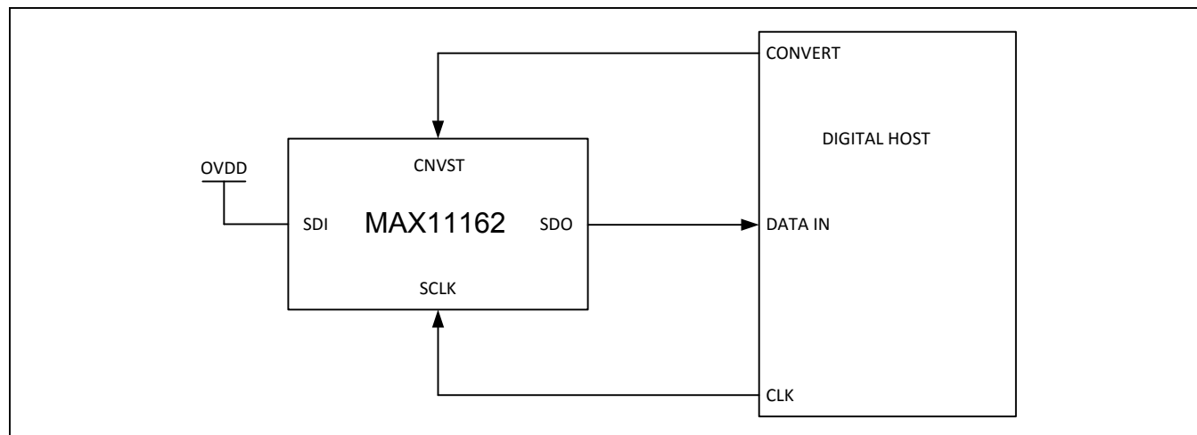
Figure 5. \overline{\text{CS}} Mode 3-Wire, No-Busy Indicator Connection Diagram (SDI High)
