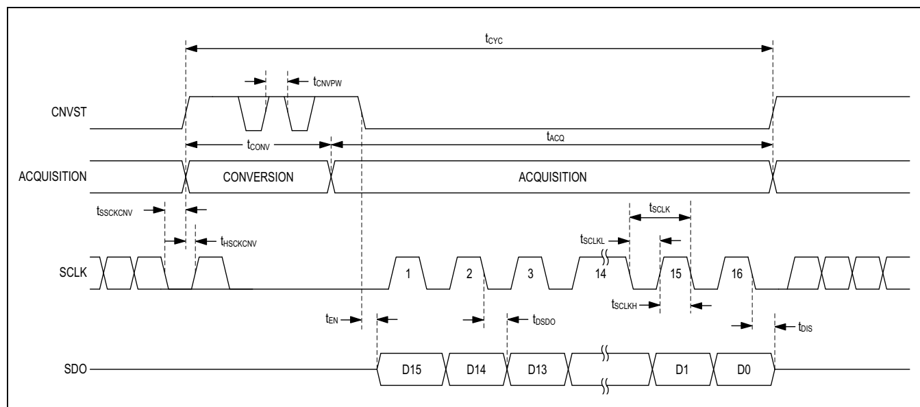
Figure 6. \overline{\text{CS}} Mode 3-Wire, No-Busy Indicator Serial Interface Timing (SDI High)
