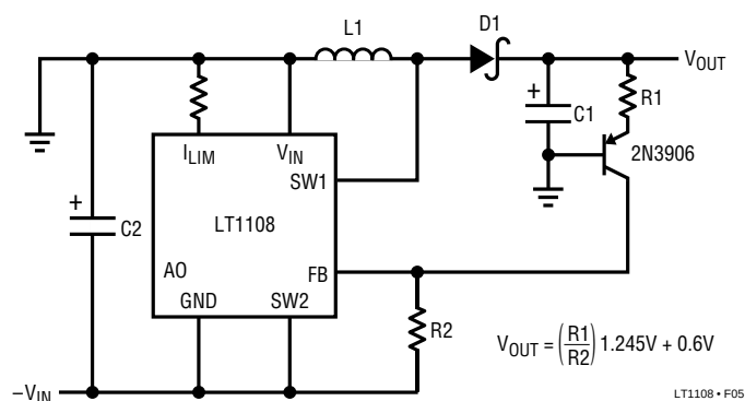
Figure 5. Negative-to-Positive Converter
