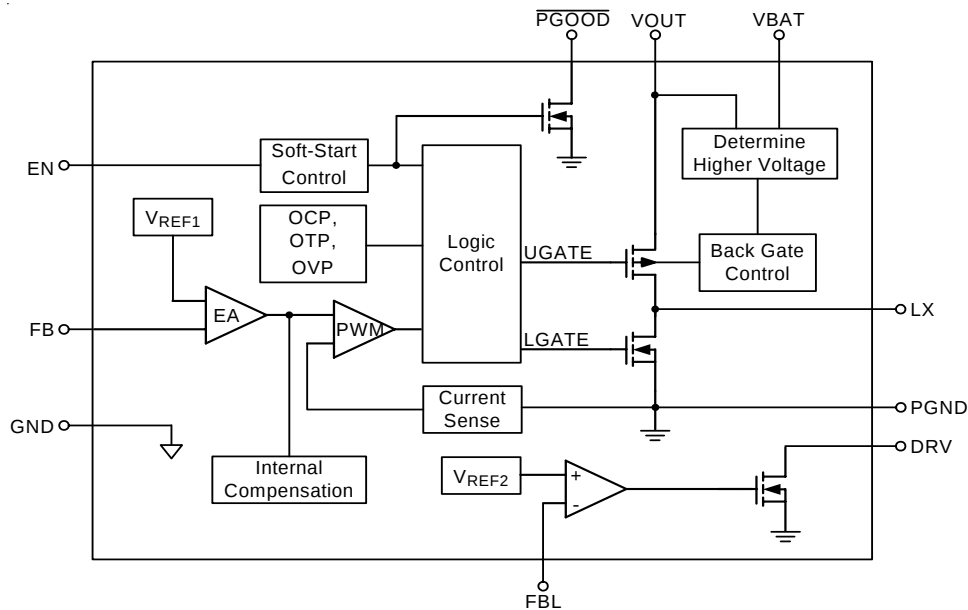
Figure 4. Adjustable Voltage Regulator
