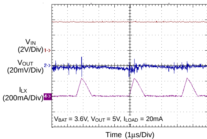
DCM Switching
