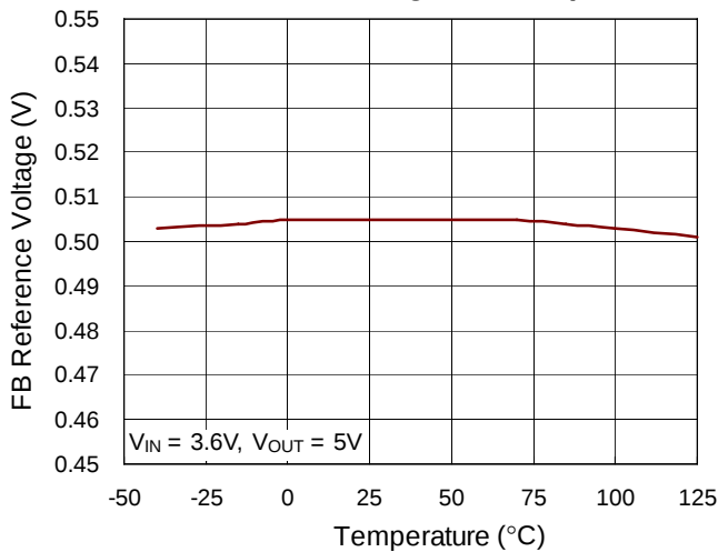
FB Reference Voltage vs. Temperature
