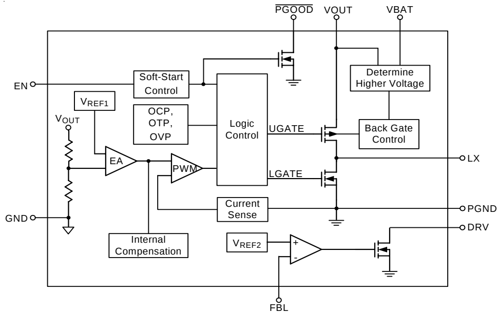
Figure 3. Fixed Voltage Regulator
