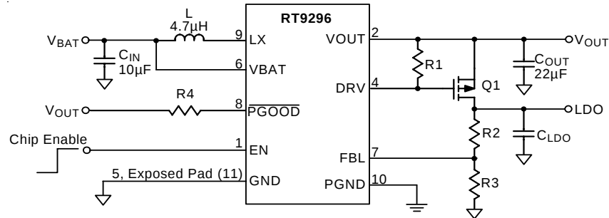
Figure 1. Fixed Output Voltage Boost Converter with Linear Regulator
