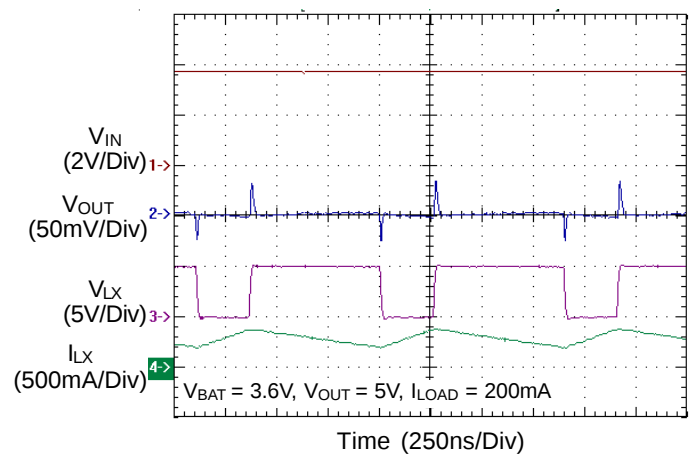
CCM Switching
