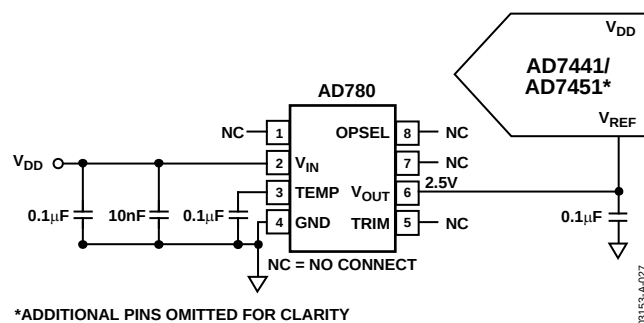
Figure 27. Typical V_{\text{REF}} Connection Diagram for V_{\text{DD}} = 5 V
