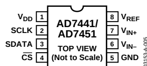
Figure 5. 8-Lead SOT-23
