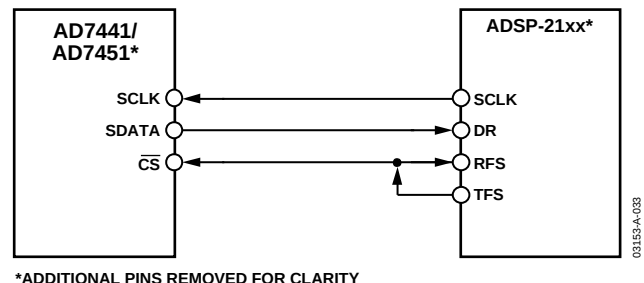
Figure 33. Interfacing to the ADSP-21xx
