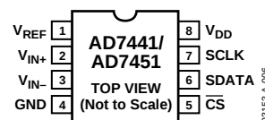
Figure 6. 8-Lead MSOP
